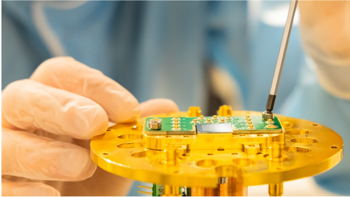
Picture 2: Impressions from the lab – multi-channel single photon detector from Pixel Photonics GmbH. © Pixel Photonics GmbH / Dr. Wladick Hartmann.
